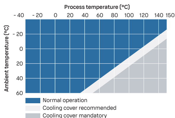
PR53GCEX process temperature
