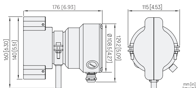
Dimensions of PR53MEX flow cell end plate bolts (integrated fittings, Flare and Pillar-type)
