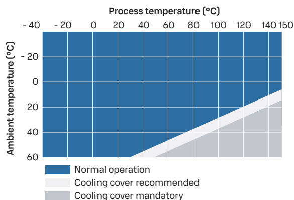
PR53GPEX process temperature
