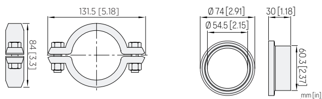
Dimensions of PR53GCEX L coupling clamp
