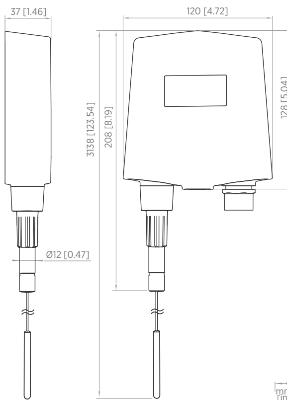
Dimensions of TMT120 and TMT130 transmitter, fixed probe model with a TMP115 probe
