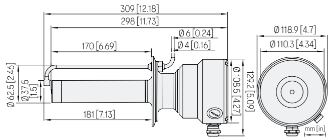
Dimensions of PR53APEX Sanitary 4", depth 170 mm, with wash nozzle
