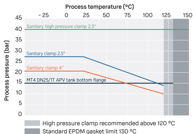
PR53APEX process pressure
