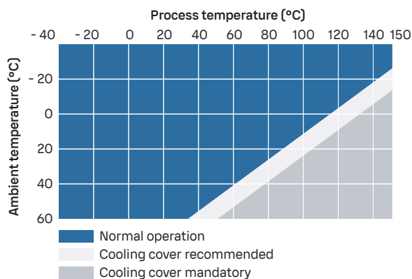
PR53APEX (depths 42 mm and 66 mm) process temperature
