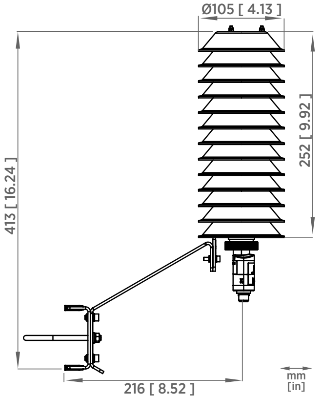
DTR503A dimensions
