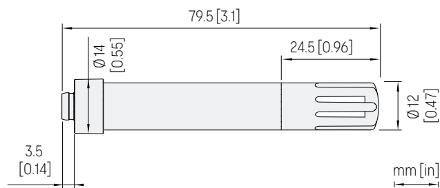
HMP113 dimensions
