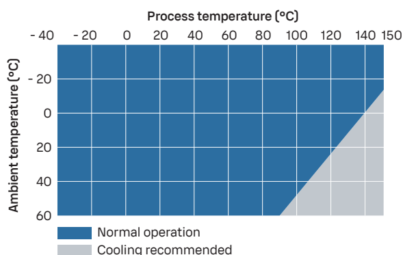
PR53AC process temperature (indicative)
