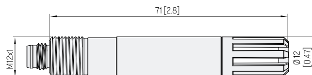
HMP110 and HMP110T probe dimensions
