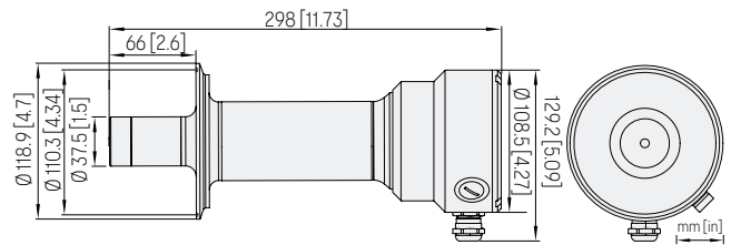
Dimensions of PR53APEX Sanitary 4", depth 66 mm
