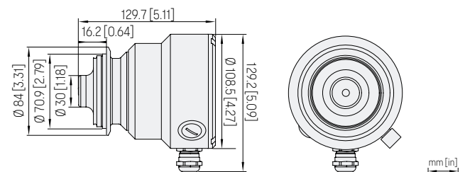
Dimensions for PR53ACEX Type N
