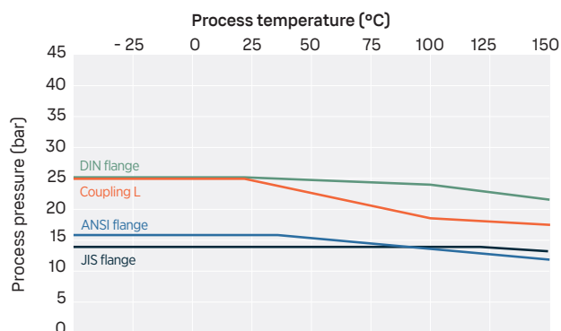
PR53GPEX process pressure
