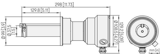
Dimensions of PR53GP L coupling 88.9 mm (3.5 inch)
