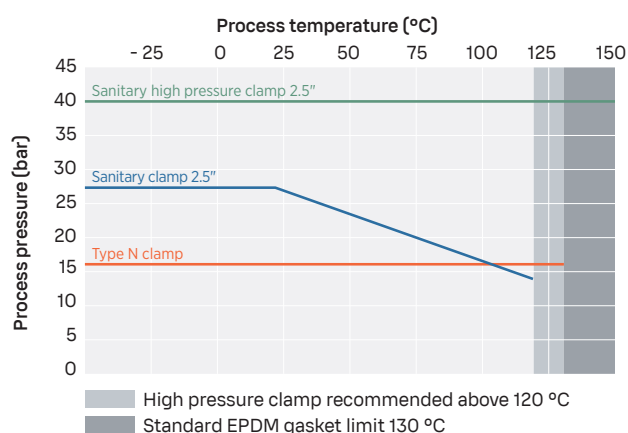
PR53ACEX process pressure
