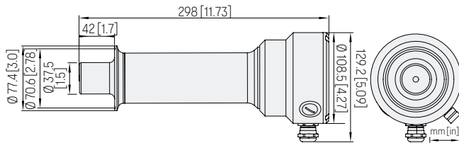
Dimensions of PR53APEX Sanitary 2.5", depth 42 mm
