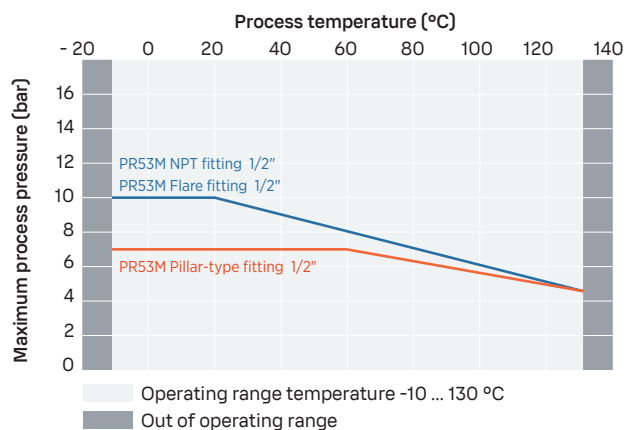
PR53MEX process pressure
