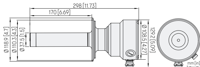
Dimensions of PR53APEX Sanitary 4", depth 170 mm
