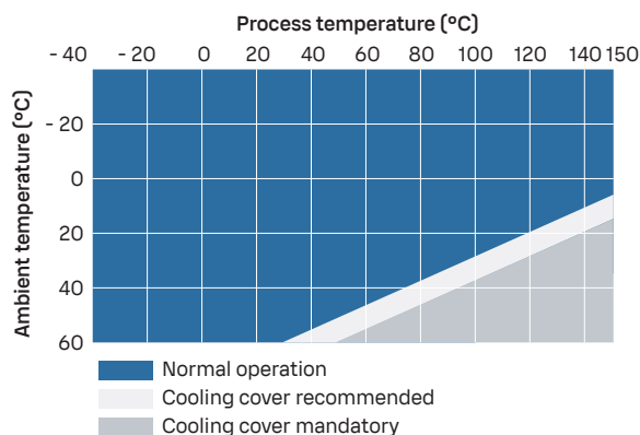
PR53APEX (depth 170 mm) process temperature
