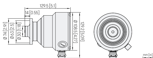
Dimensions of PR53GCEX
