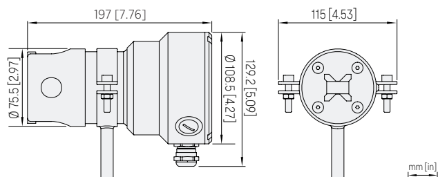
Dimensions of PR53MEX flow cell end plate bolts (NPT fitting)
