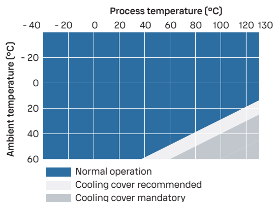
PR53MEX process temperature
