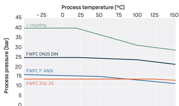
PR53GCEX process pressure
