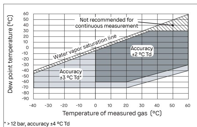
Dew point measurement accuracy vs. measurement conditions
