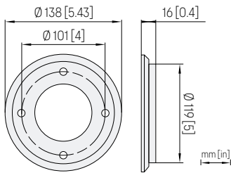
Dimensions of PR53AP tank bottom welding flange
