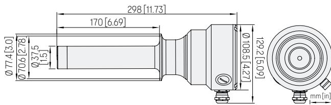
Dimensions of PR53APEX Sanitary 2.5", depth 170 mm
