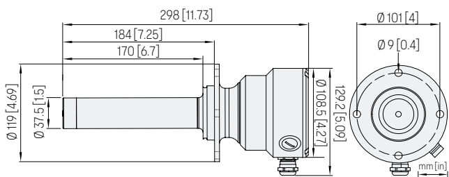
Dimensions of PR53APEX tank bottom flange, depth 170 mm
