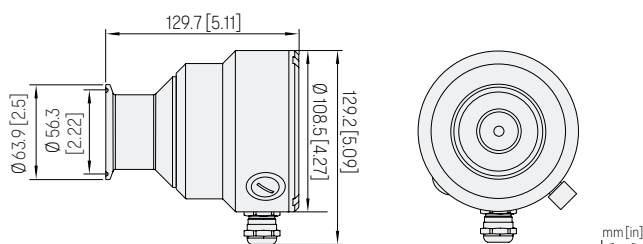
Dimensions for PR53ACEX Sanitary 2"
