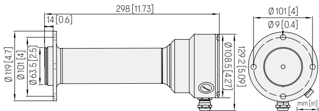
Dimensions of PR53APEX tank bottom flange, flush-mounted
