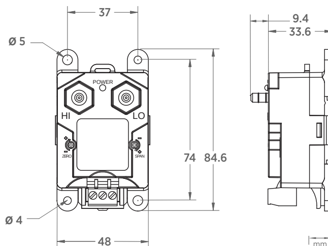
PDT101 dimensions
