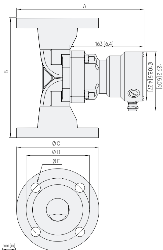
Dimensions of PR53WEX valve body
