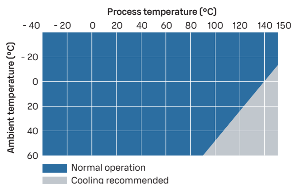
PR53AP, depth 170 mm process temperature (indicative)
