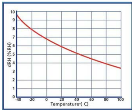
Measurement error at 100 %RH at various temperatures when the temperature difference between the ambient air and the sensor is 1 °C
