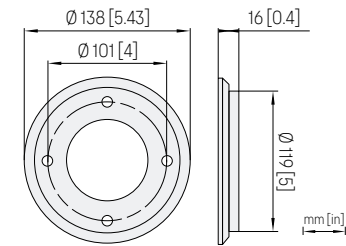
Dimensions of PR53APEX tank bottom welding flange
