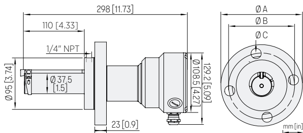
Dimensions of PR53GPEX 2" flange
