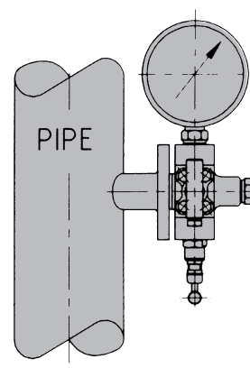
VERTICAL PIPING PRESSURE MEASUREMENT
