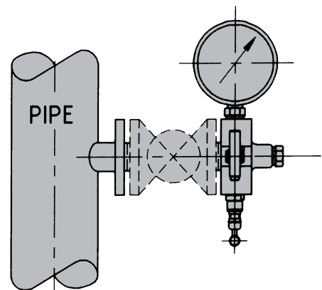
VERTICAL PIPING PRESSURE MEASUREMENT
