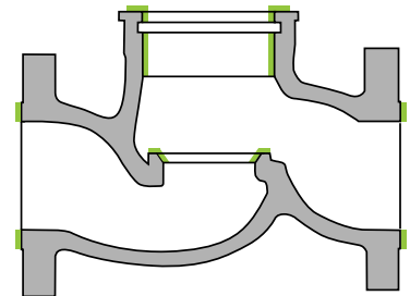
Machinable faces
